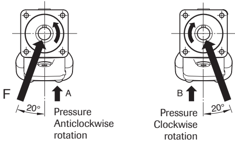
Optimal force direction of radial load
