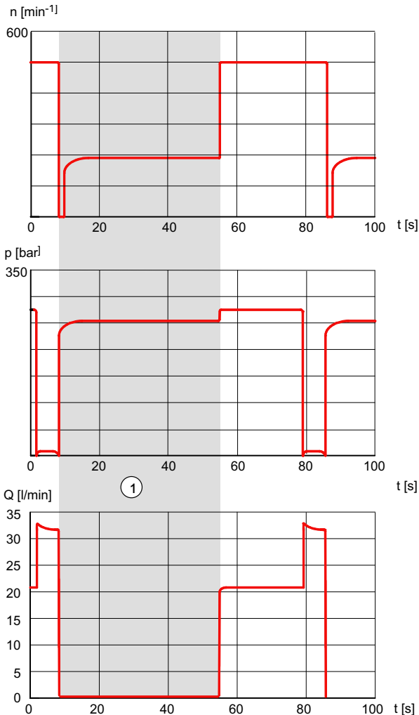
Pump QX53-063 with viscosity 20 mm 2 /s
