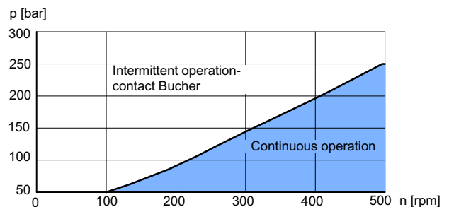
Pump QX53-063 measured with viscosity 42 mm 2 /s
