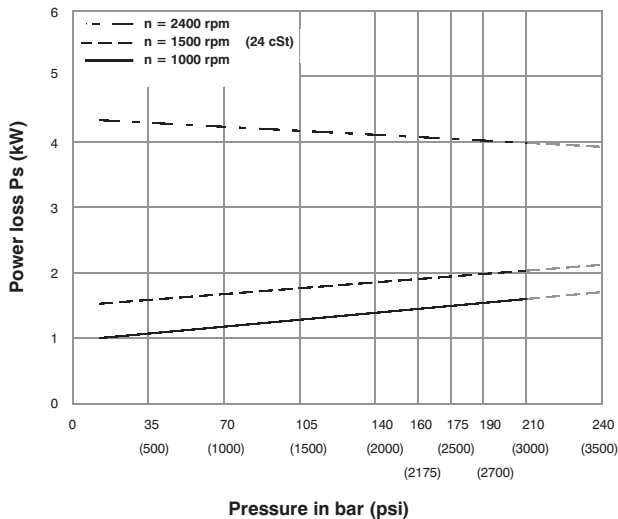
HYDROMECAHNICAL POWER LOSS (TYPICAL)
